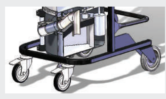
Tank with liquid abatement system to inertising reactive dust
